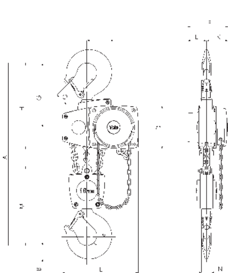
Yalelift 360, 10000 kg, three falls
