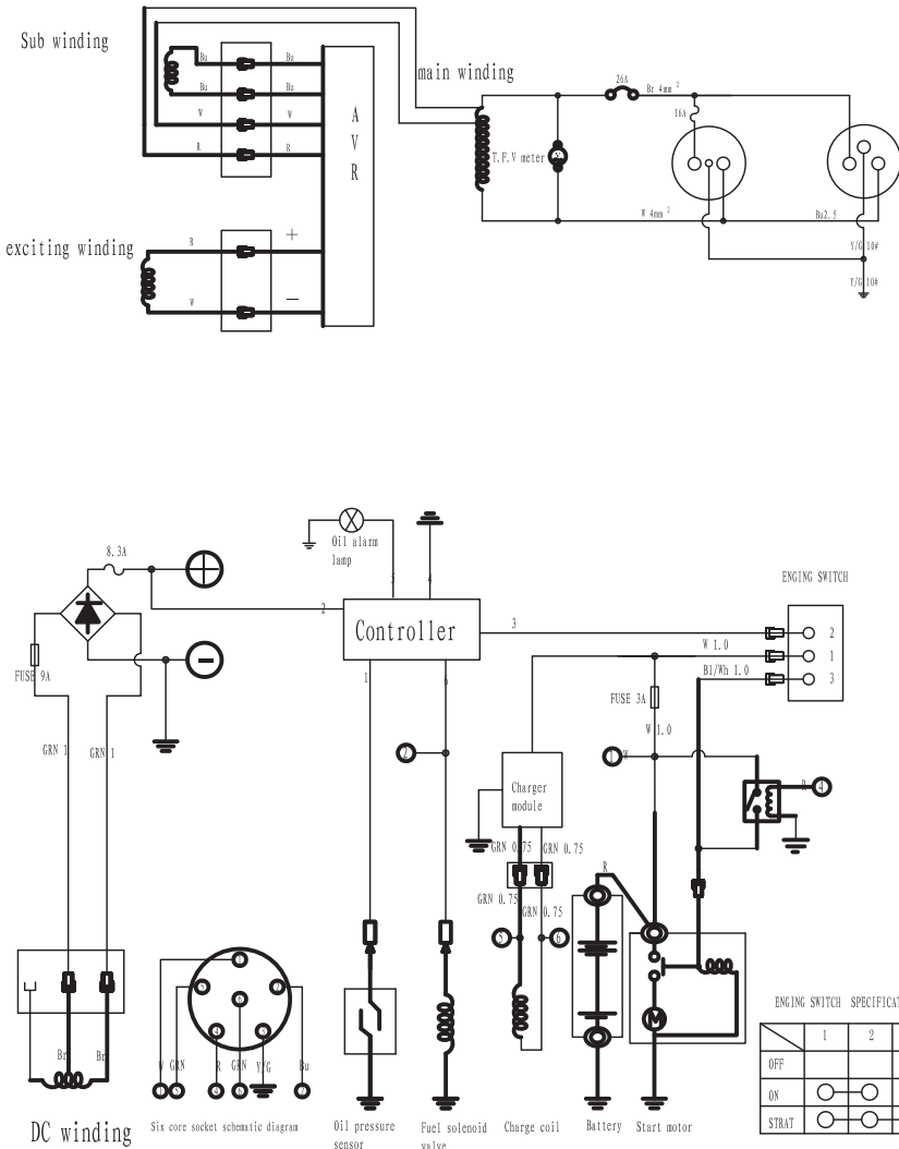
Figure 5-1 Schéma circuit mono voltage monophasé
